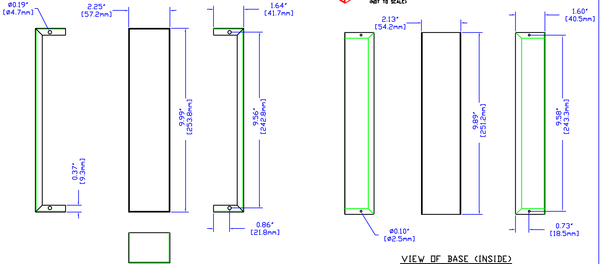
VIEW OF LID (INSIDE)
