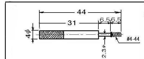
LONG SCREW: STEEL IN NICKEL PLATED (2 pcs)
