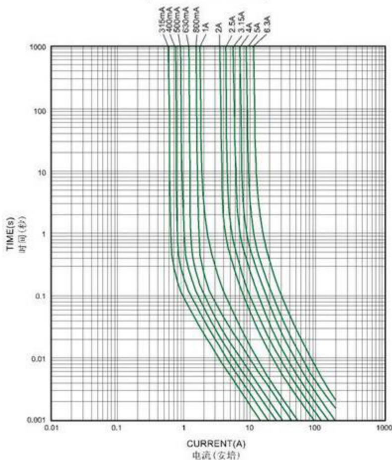
5RF AVERAGE I-T CHARACTERISTICS CURVE (FOR REFERENCE)
