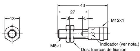
E2A-S08KS02-M1-□□
