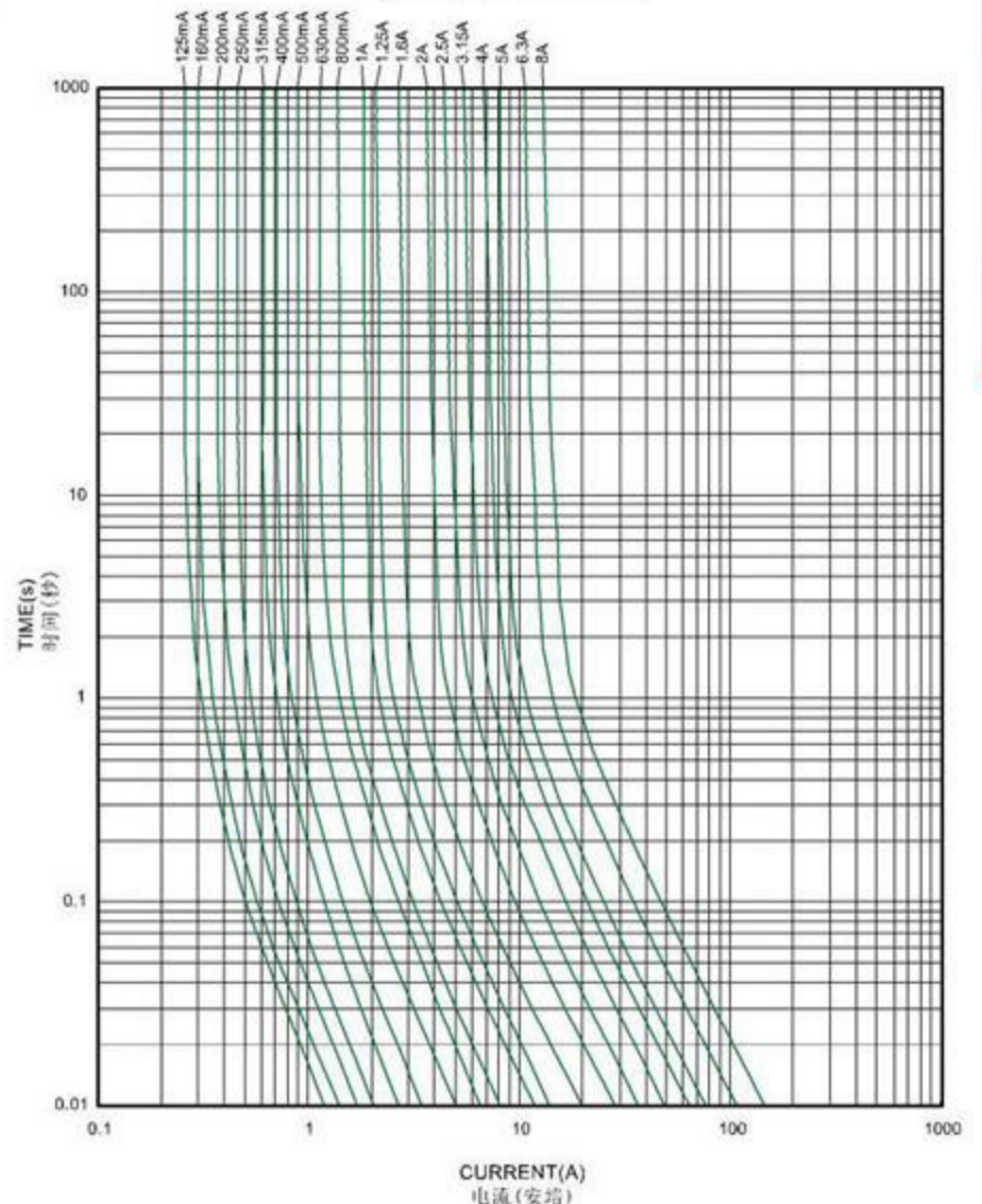
50F 平均 I-T 曲线图 (仅供参考) 50F AVERAGE I-T CHARACTERISTICS CURVE (FOR REFERENCE)
