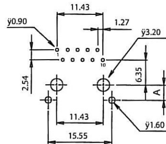
PC Board Layout Ref.
