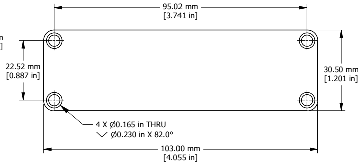
END PLATE
