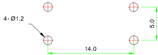
PCB DIMENSION
