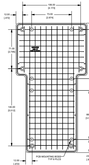
FRONT VIEW OF BOX
