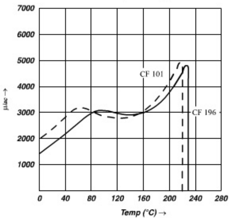
Initial Permeability Vs Temperature
