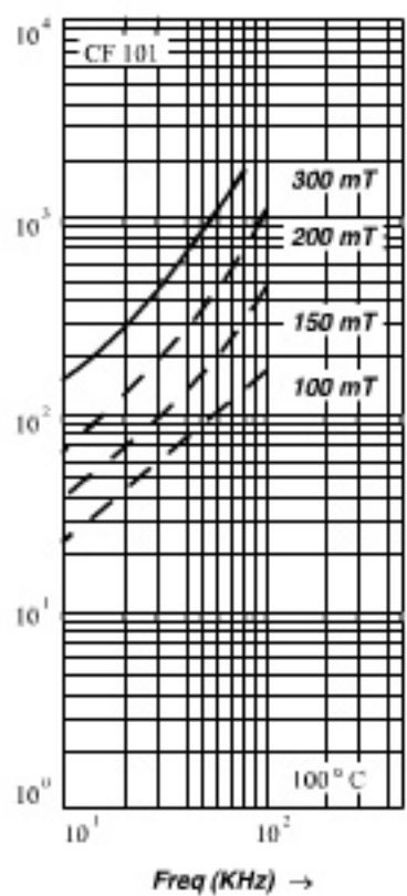
Core loss Vs Frequency
