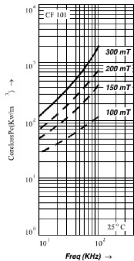
Core loss Vs Frequency
