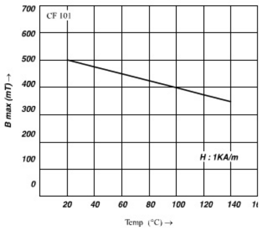
Flux density Vs Temperature
