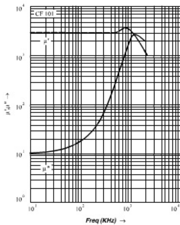
Complex Permeability Vs Frequency
