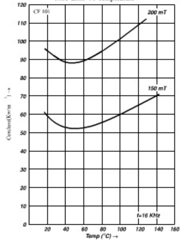
Core Loss Vs Temperature
