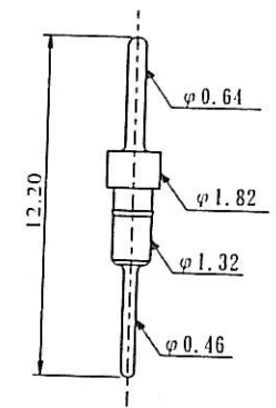
DIMENSION TABLE
