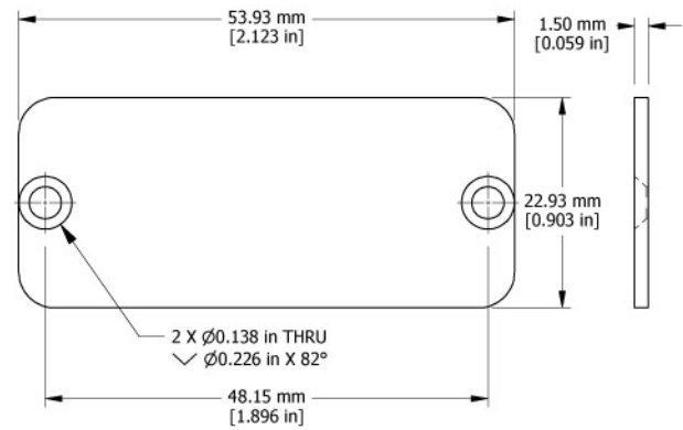
END PLATE
