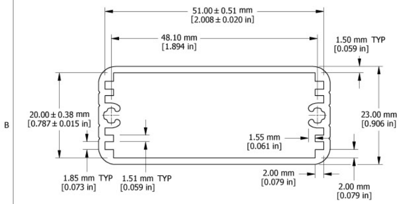
EXTRUSION
