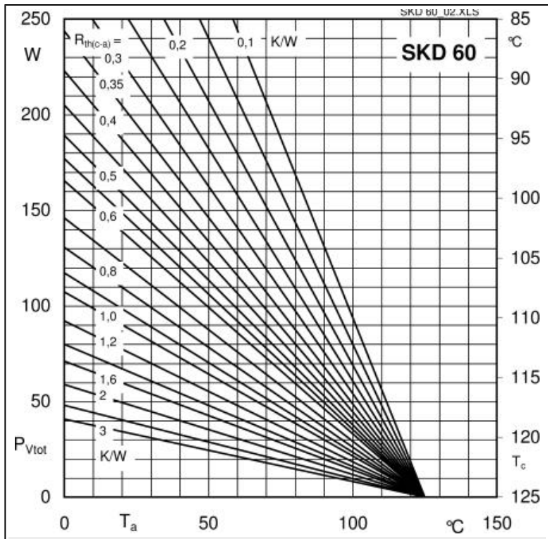
Fig. 3R Power dissipation vs. case temperature
