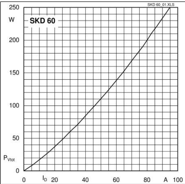
Fig. 3L Power dissipation vs. output current
